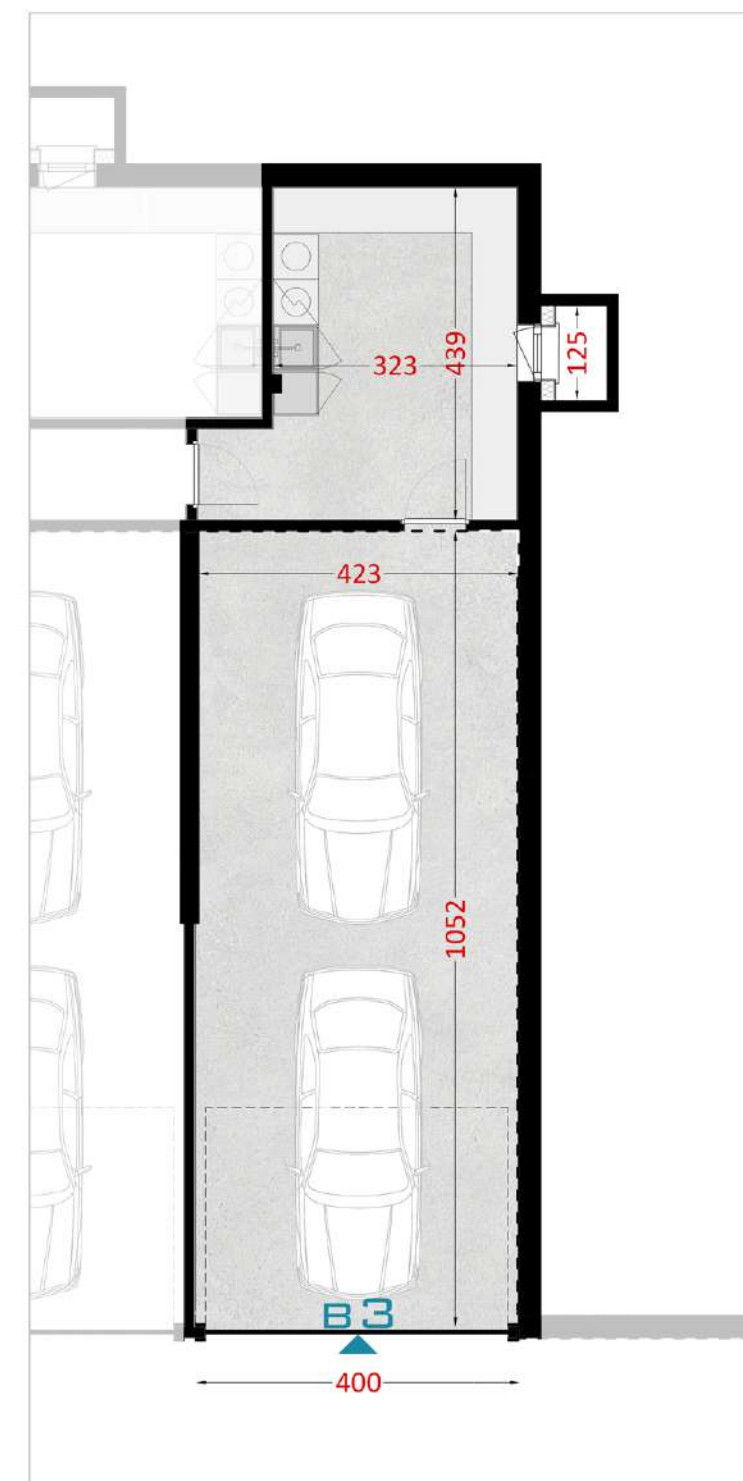
piano interrato
