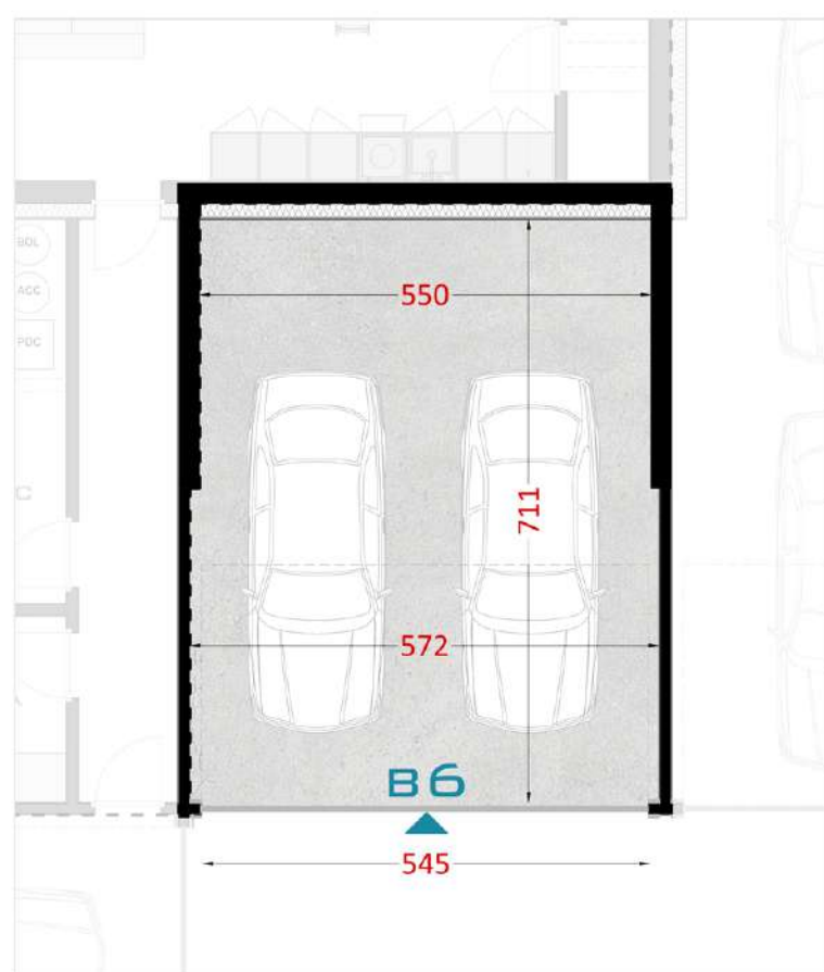
piano interrato
