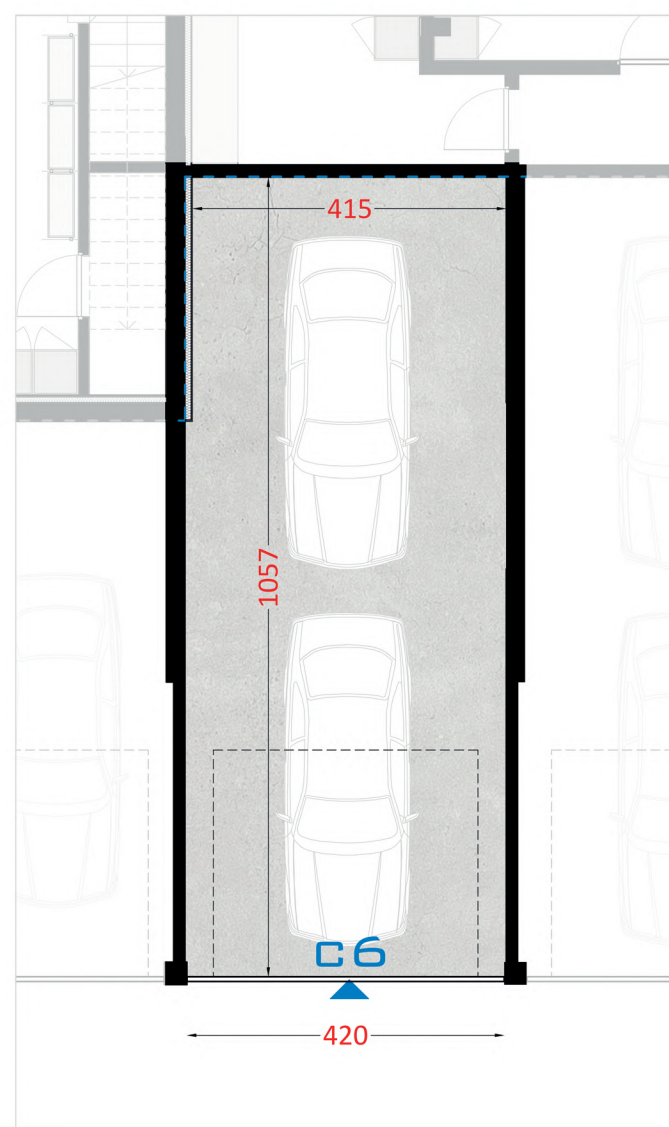
piano interrato
