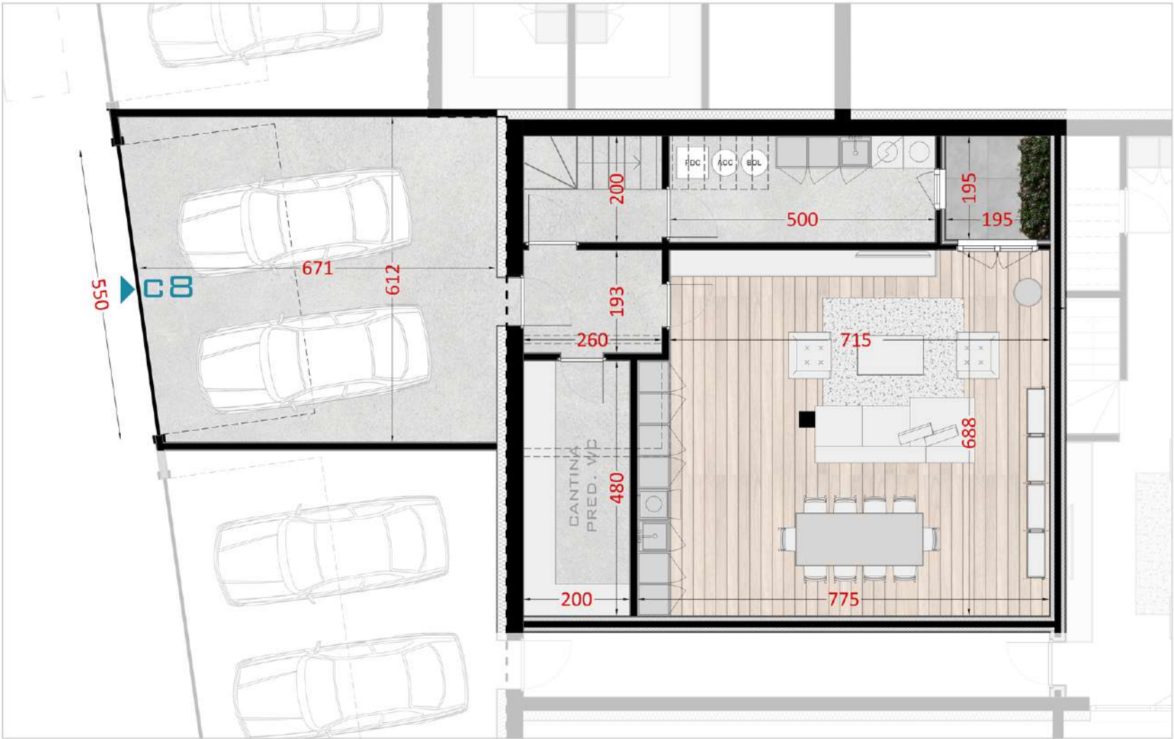
piano interrato
