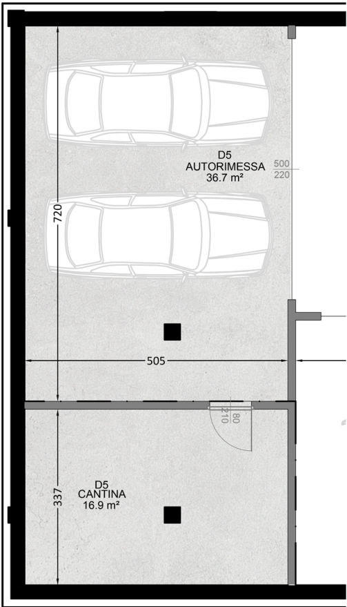
piano interrato
