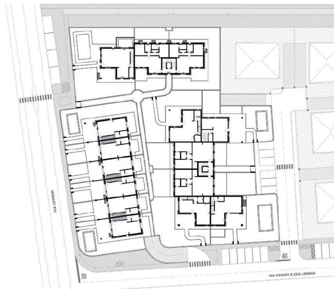
PIANO TERRA
