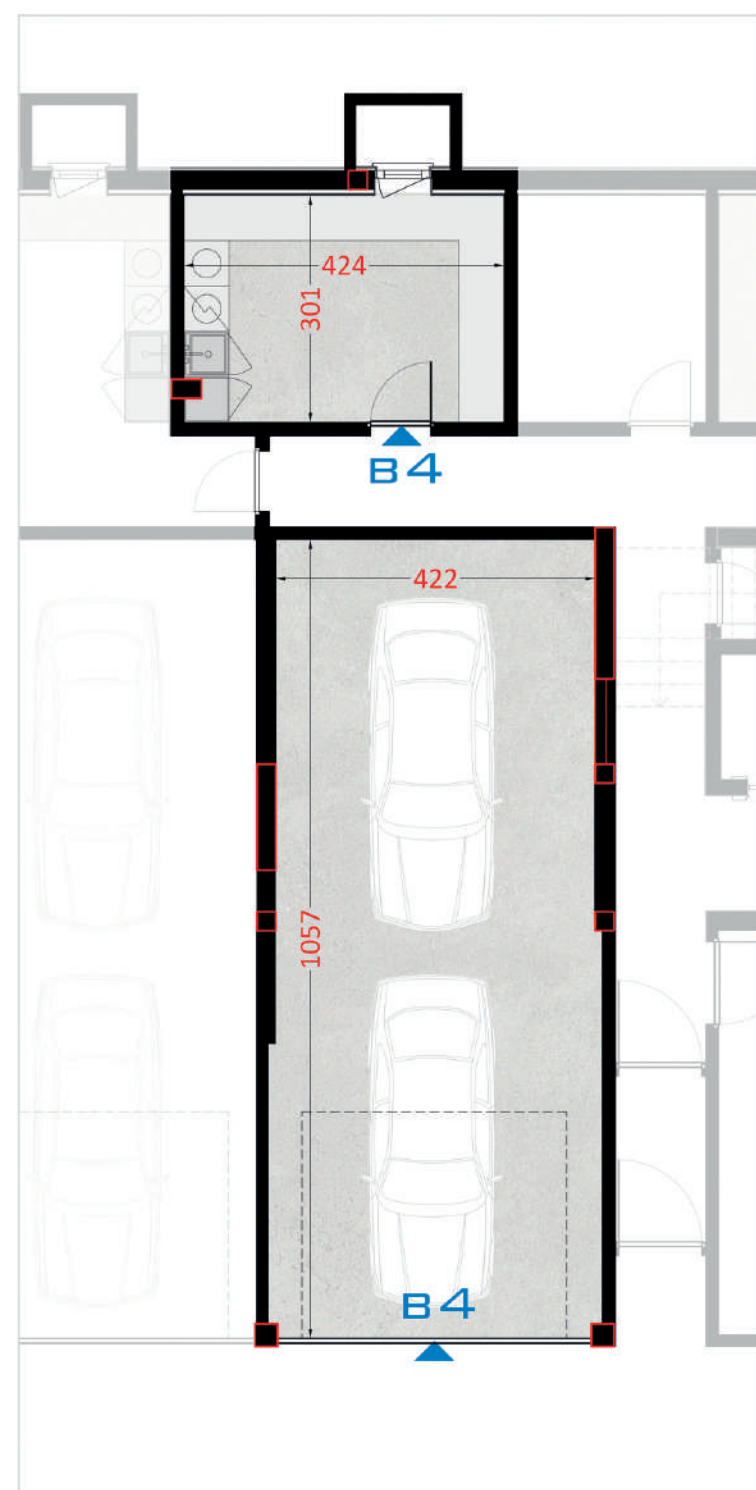
piano interrato
